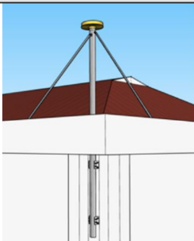
MONUMENTATION SKETCH
